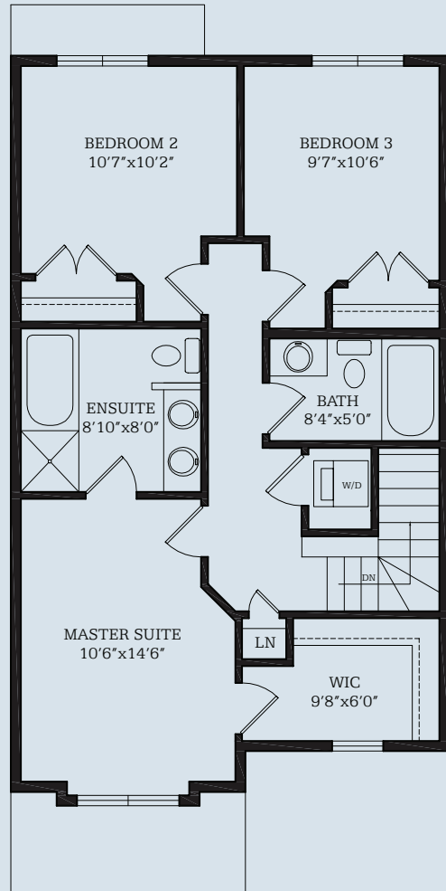
UPPER FLOOR PLAN 729 SQ.FT.
