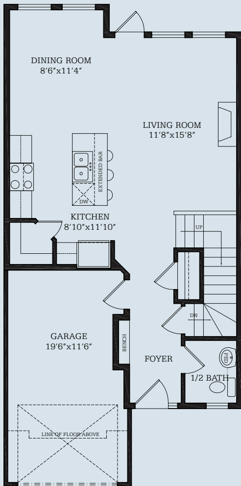
MAIN FLOOR PLAN 626 SQ.FT.
