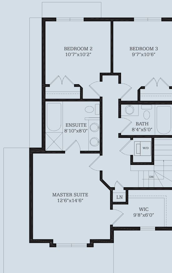
UPPER FLOOR PLAN 759 SQ.FT.
