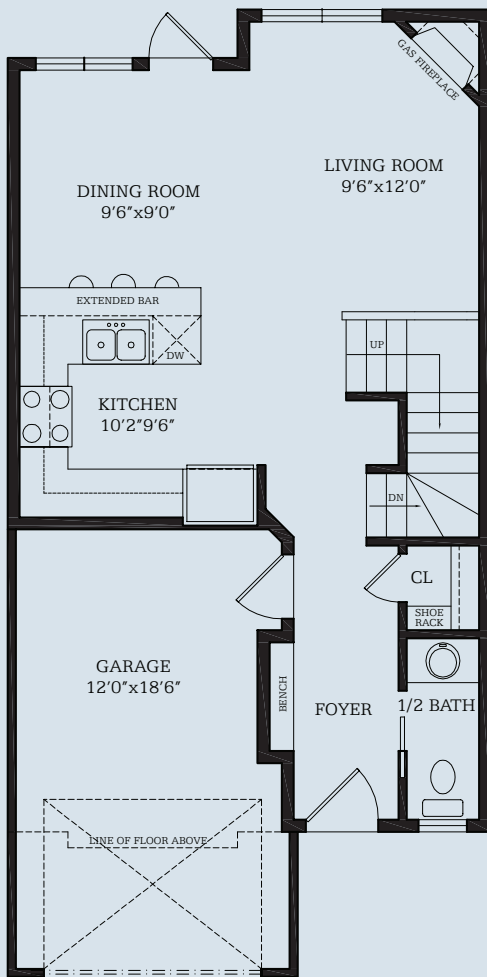
MAIN FLOOR PLAN 525 SQ.FT.
