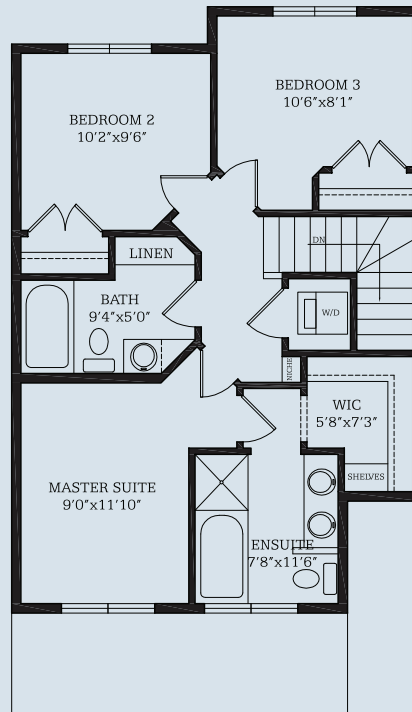
UPPER FLOOR PLAN 633 SQ.FT.
