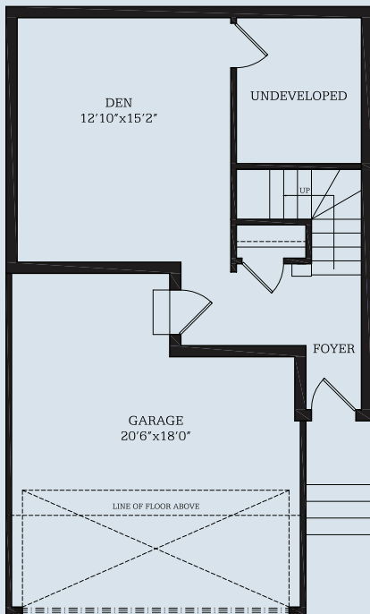
LOWER FLOOR PLAN (with drive-under garage) 186 SQ.FT.
